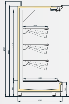
VINSON MT/F&V 1100/H2200
