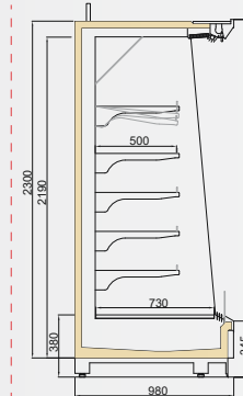
VINSON MT/FV 1000/H2200
