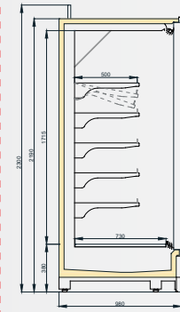
VINSON MT DGD/T55 1000/H2200
