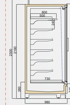
VINSON DGD/VNZ 1000/H2200
