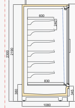
VINSON DGD/VNZ 1100/H2200
