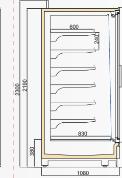
VINSON DGD/VWL 1100/H2200
