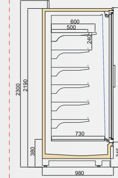
VINSON DGD/VWL 1000/H2200
