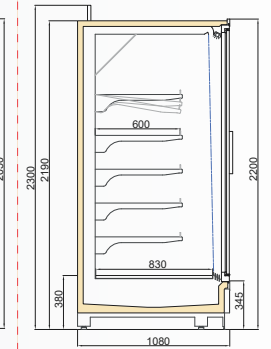
VINSON MT DGD/VWL 1100/H2200
