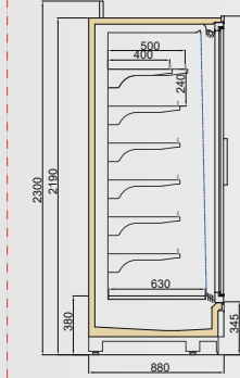
VINSON DGD/VWL 900/H2200
