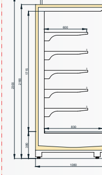
VINSON DGD/T55 1100/H2200
