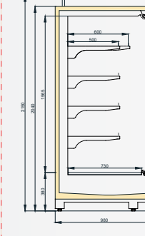
VINSON DGD/T55 1000/H2050
