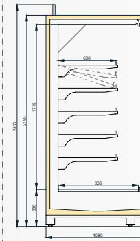
VINSON MT DGD/T55 1100/H2200
