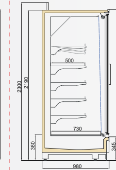
VINSON MT DGD/VWL 1000/H2200
