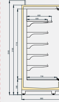
VINSON DGD/T55 1000/H2200
