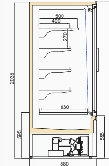
LISTER DGD/VNZ 900/H2050
