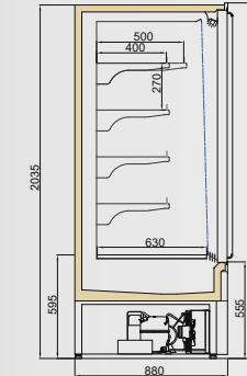
LISTER DGD/T55 900/H2050
