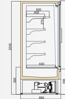
LISTER DGD/VWL 900/H2050
