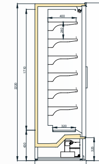
MARAS TKY 750/H2200
