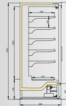
MARAS SLD 750/H2050
