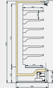
MARAS DP PLUS 900/H220C
