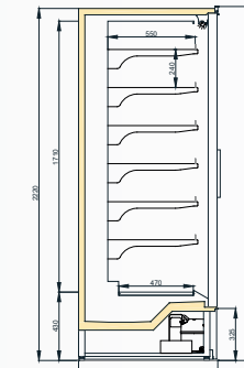
MARAS TKY 900/H2200
