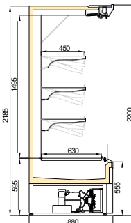
LISTER MT/F&V 900/H2200
