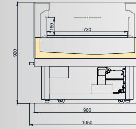
FIELD 1000 FG
