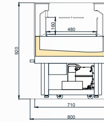
FIELD 800 FG
