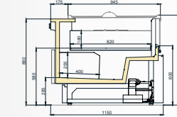
HAWKES 800 FG/SS SLD
