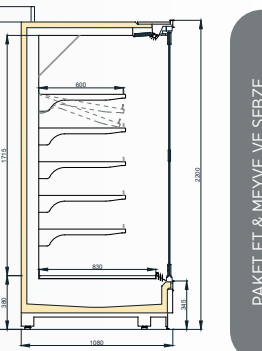
VINSON MT DGD/SGD 1100/H2200
