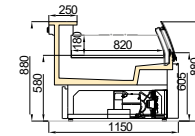
PARRY DP CG 800 H1500
