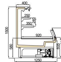
PARRY FISH CG 900
