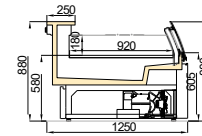
PARRY DP CG 900 H1500
