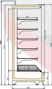
FOSTER SKY 900/H2200
