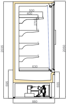
LISTER DGD/VNZ 900/H2050
