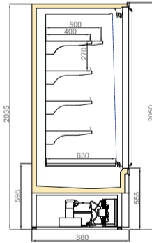
LISTER DGD/T55 900/H2050
