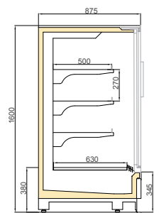
TAKAHE DGD/SKY 900/H1600
