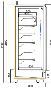
VINSON DGD/T55 900/H2200
