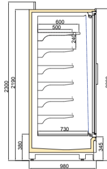
VINSON DGD/VNZ 1000/H2200
