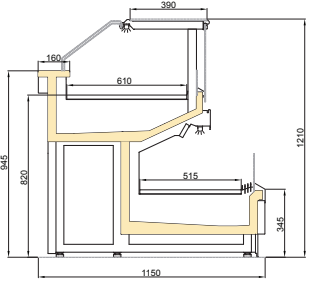
CUPOLA FG
